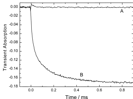
Fig. 4. Time traces of bleaching at 505 nm of 30 \mu\text{M} \beta -carotene and 1.75 M o -cresol (A) or 1.75 M phenol (B) in di- tert -butylperoxide/benzene (7:3, v/v) after laser flash photolysis at 355 nm.
